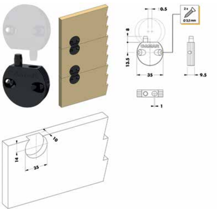
Paneelverbinding type 814.00.P2.00.01
